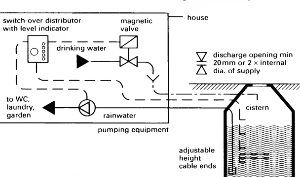
12 Drinking water supplementary supply
